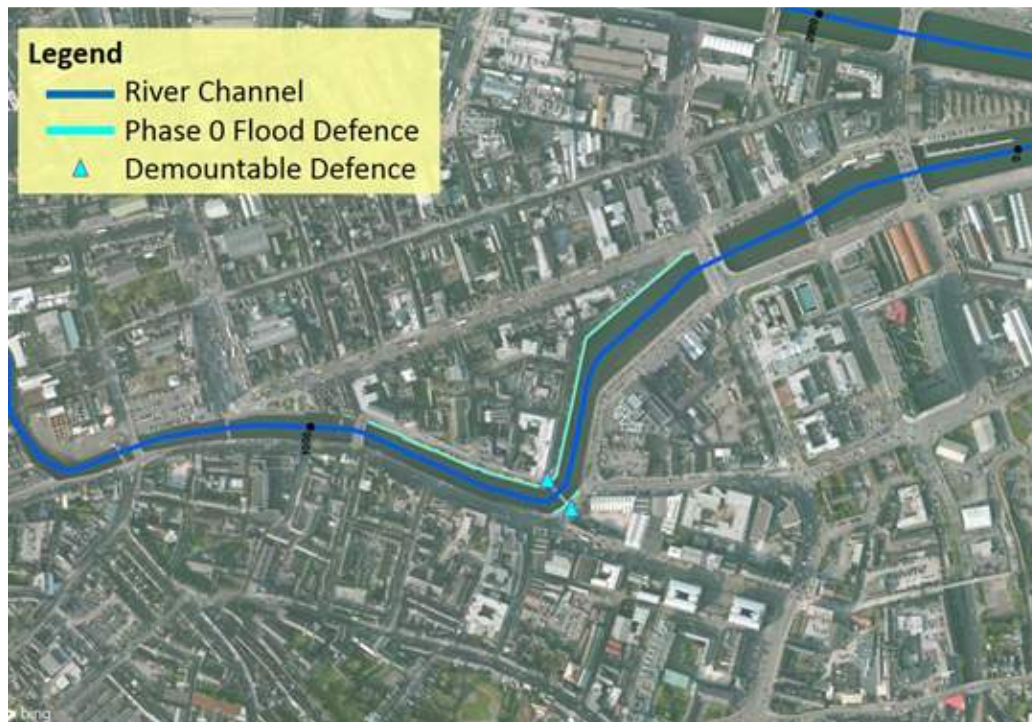
Figure 22: Defence lines for Morrison's Island
