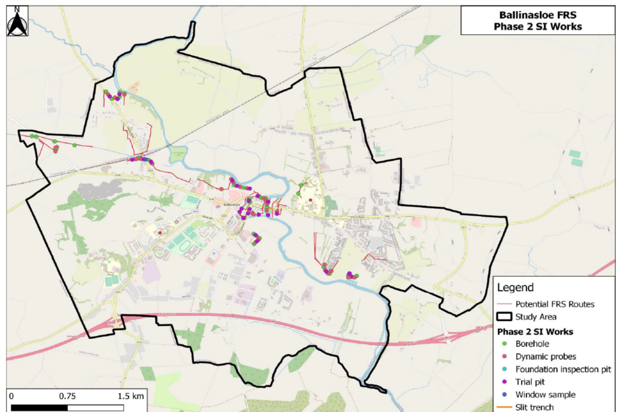
Figure 3.2: Location of the 88 No. Phase 2 SI works along with the potential FRS measures (Basemap: OSM).
