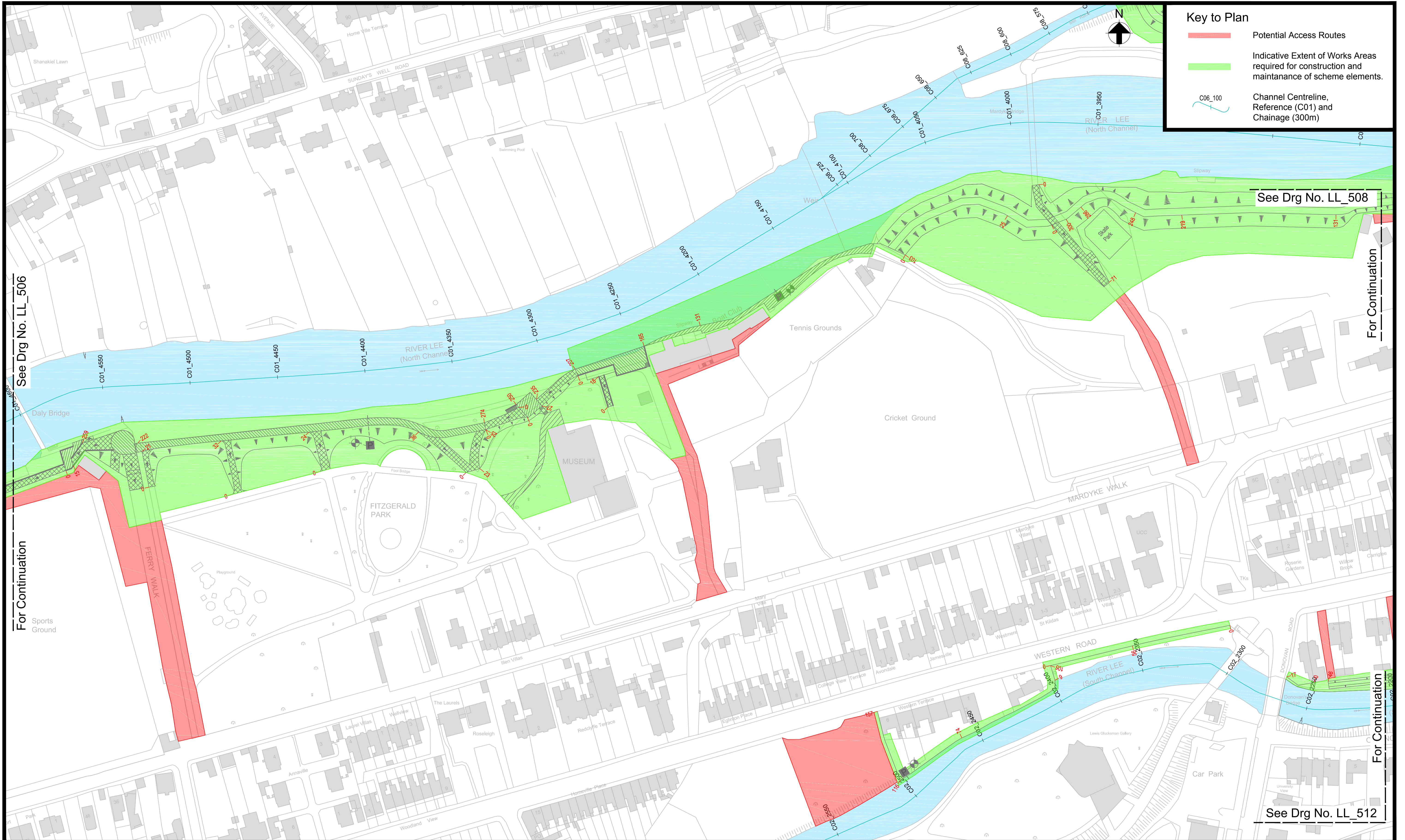
Drg. No. LL_507 Possible Access Routes and Works Areas (Sheet 7 of 15)
