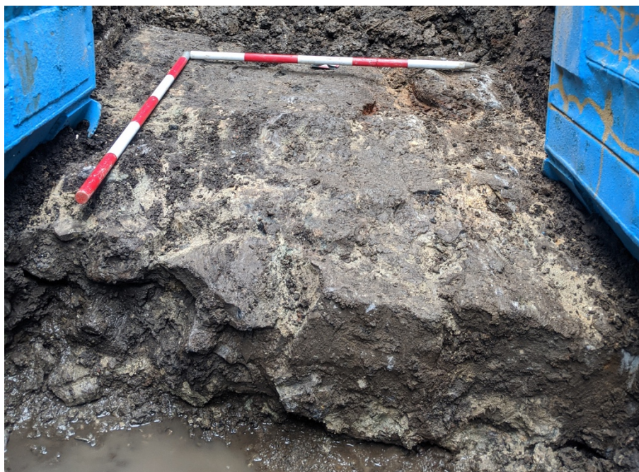
Figure 39 Wall in TT5-1A (C5-1A-15), view facing south
