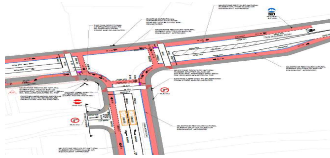
Fig.3-R639 / Hazelwood Junction Proposed Layout
